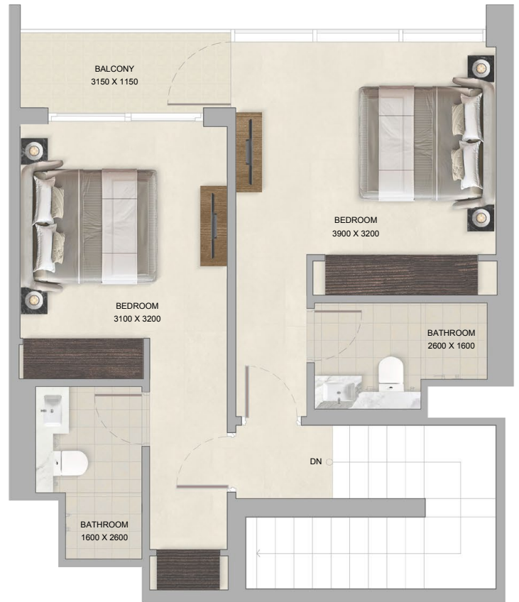
UPPER LEVEL
